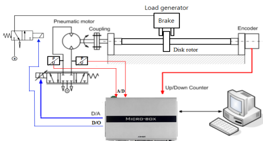
[Fig. 2] Layout of the experimental devices
