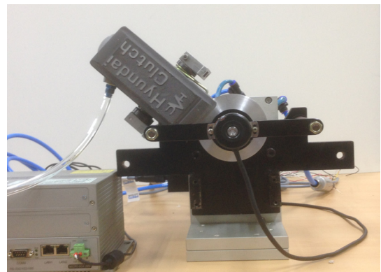
[Fig. 3] Pneumatic motor Drive system
