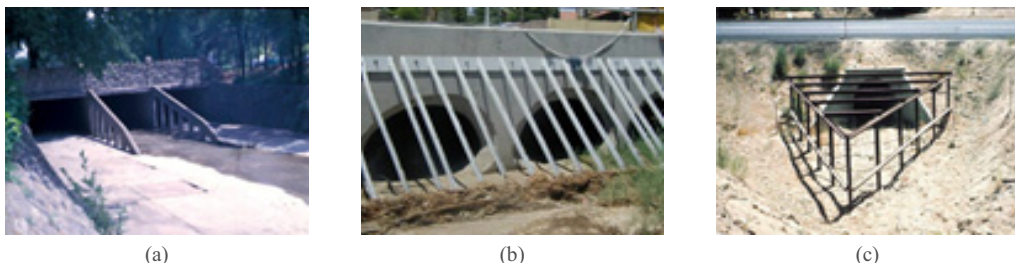
Fig. 1. Debris Reduction System(FHWA, 2005) (a) debris fins (b) debris racks (c) debris deflectors
